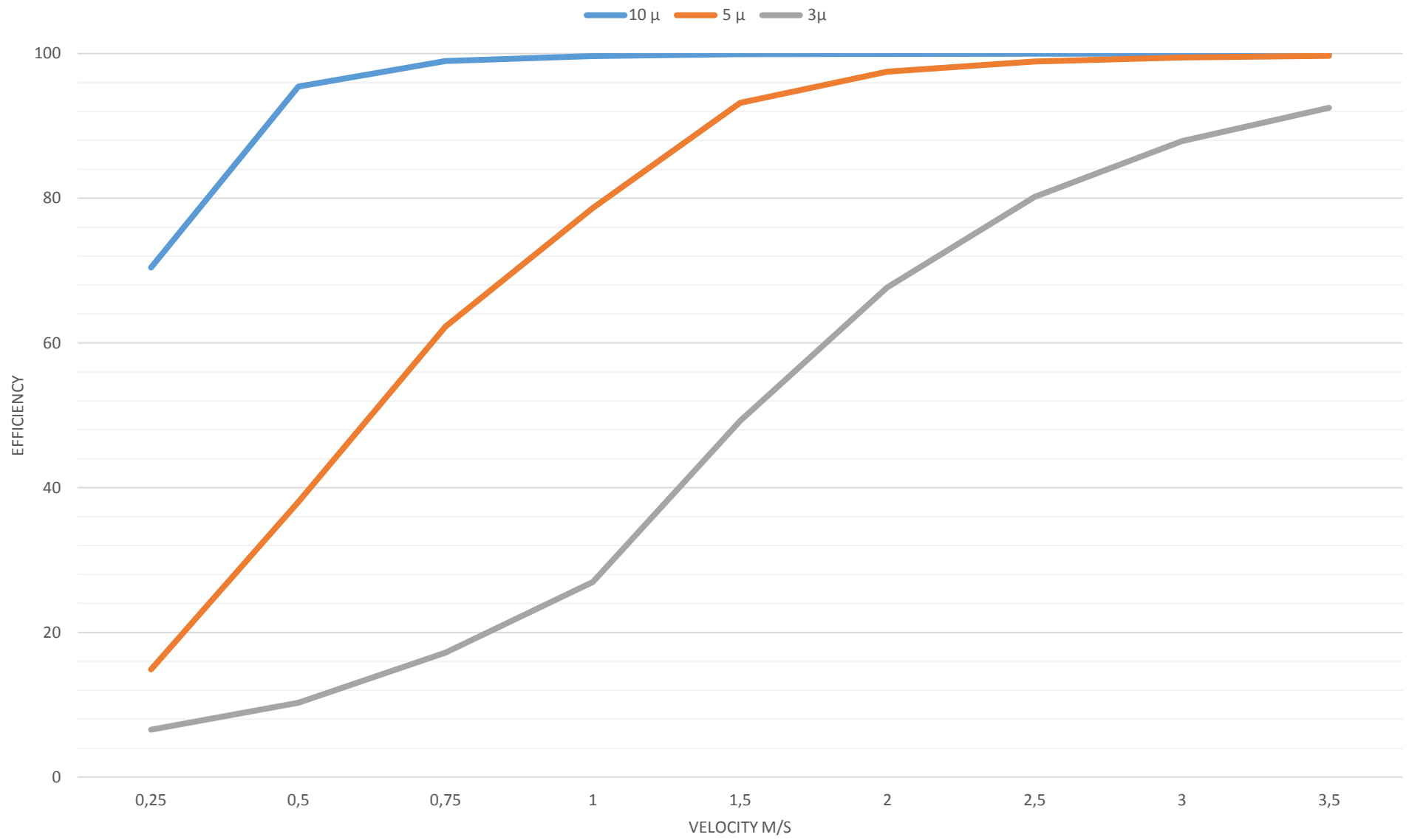
Efficiency in function of velocity and droplet size for BlueFil® MX99-5
