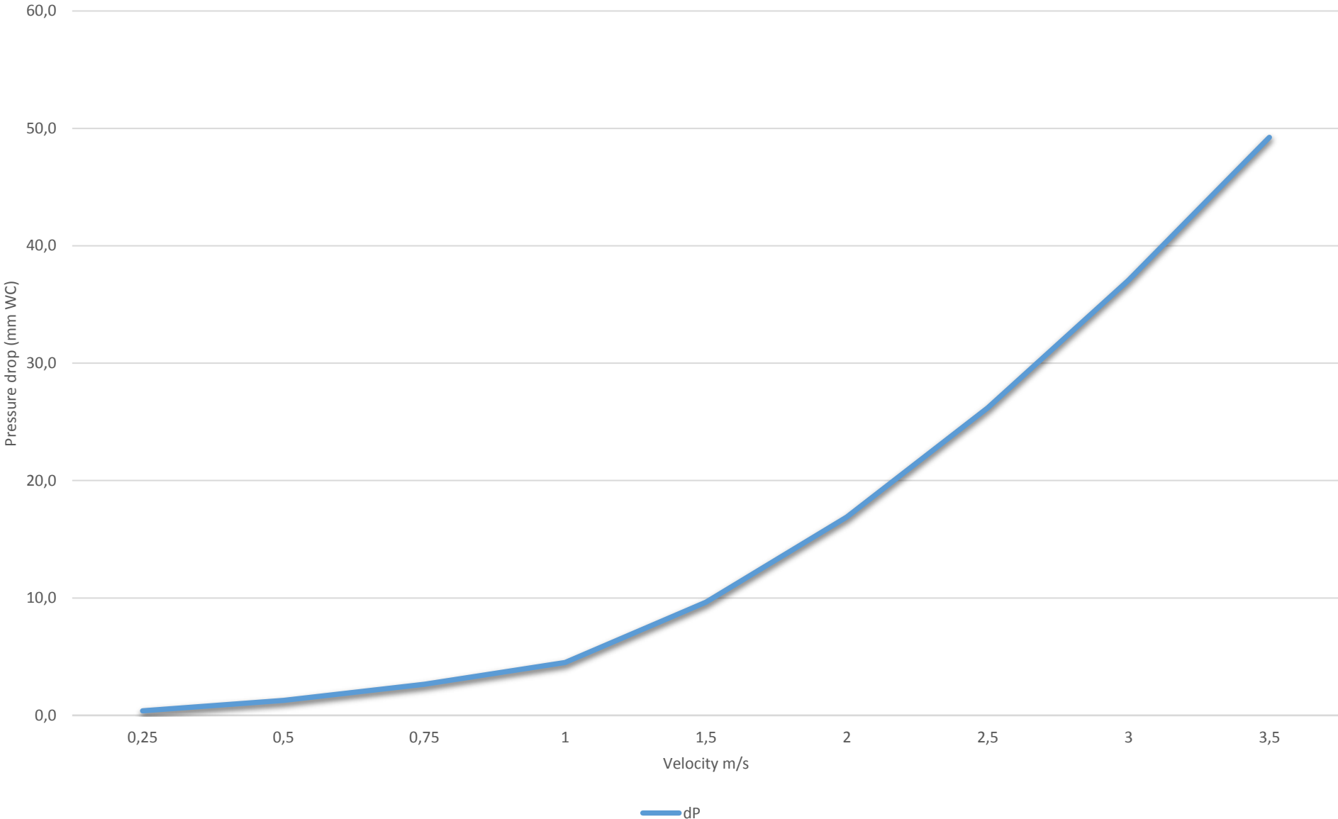
Pressure drop in function of velocity BlueFil® MX 99-5
