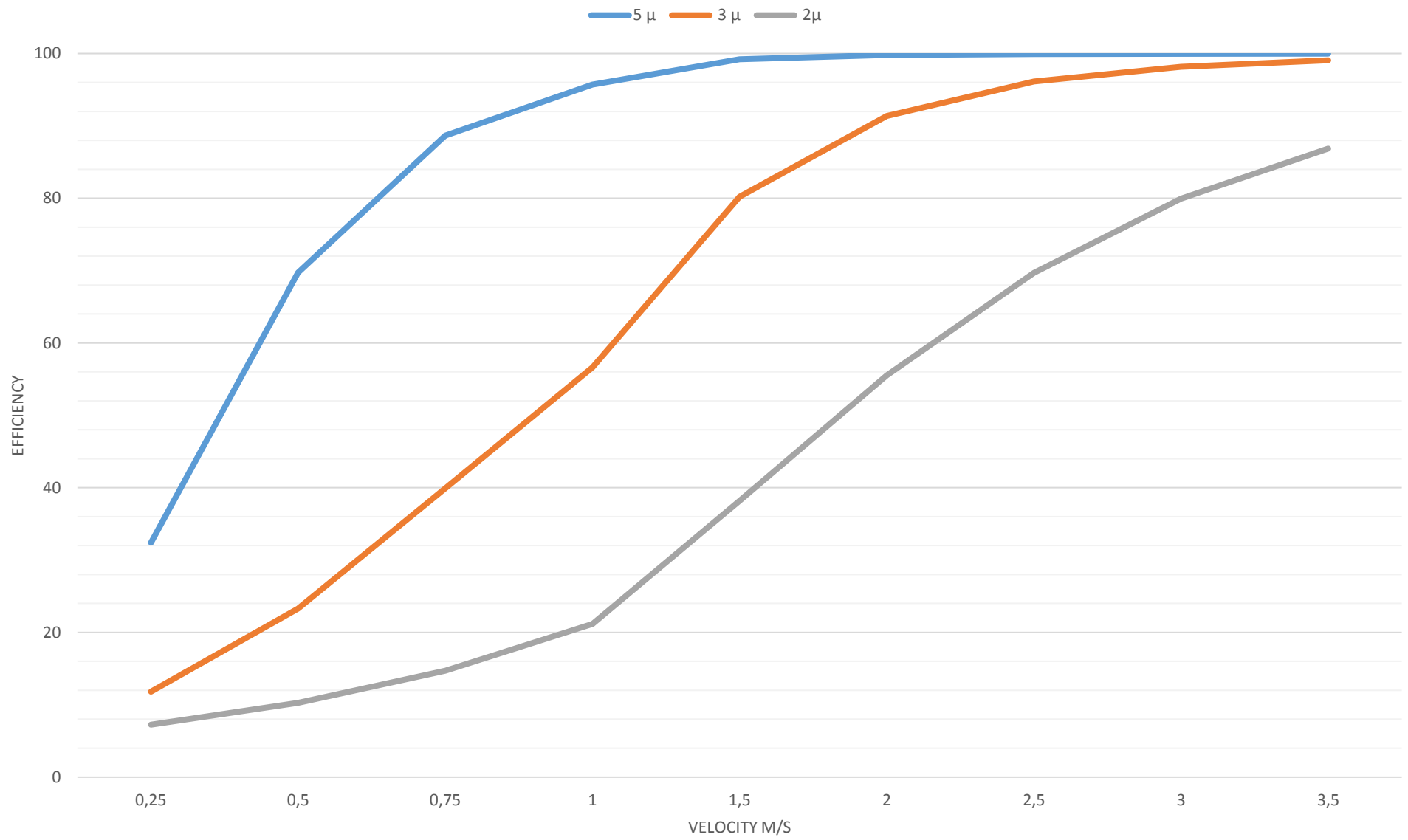
Efficiency in function of velocity and droplet size for BlueFil® MX99-3
