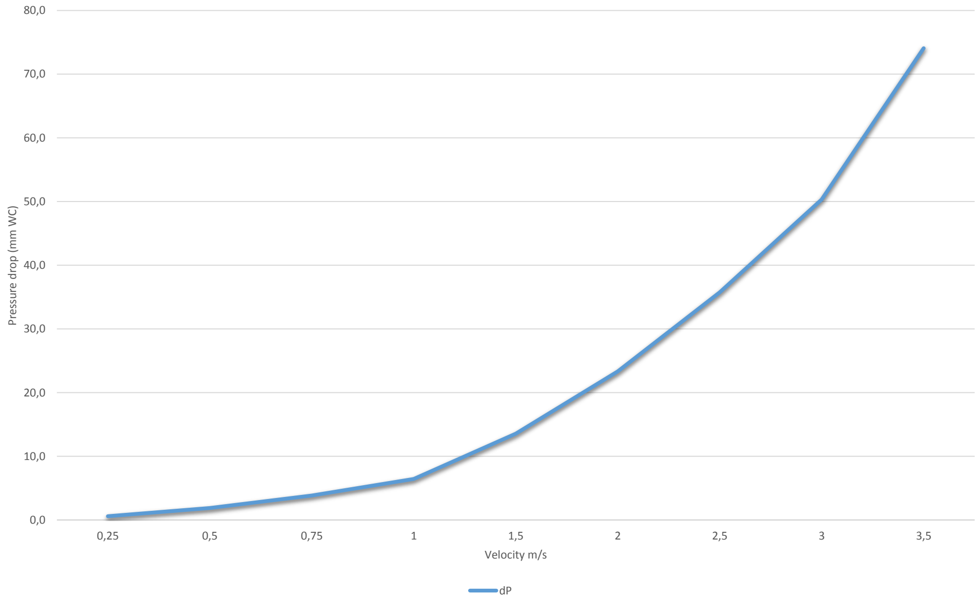
Pressure drop in function of velocity for BlueFil® MX99-3
