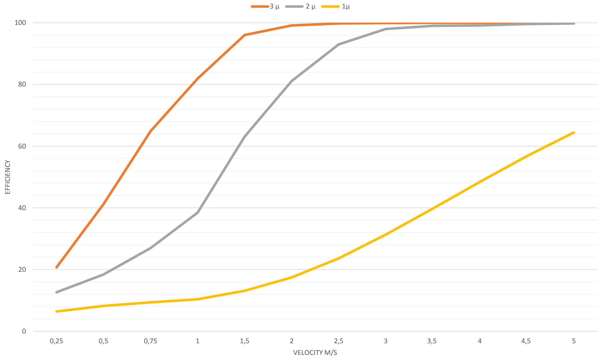
Efficiency in function of velocity and droplet size for BlueFil® MX99-2 \mu
