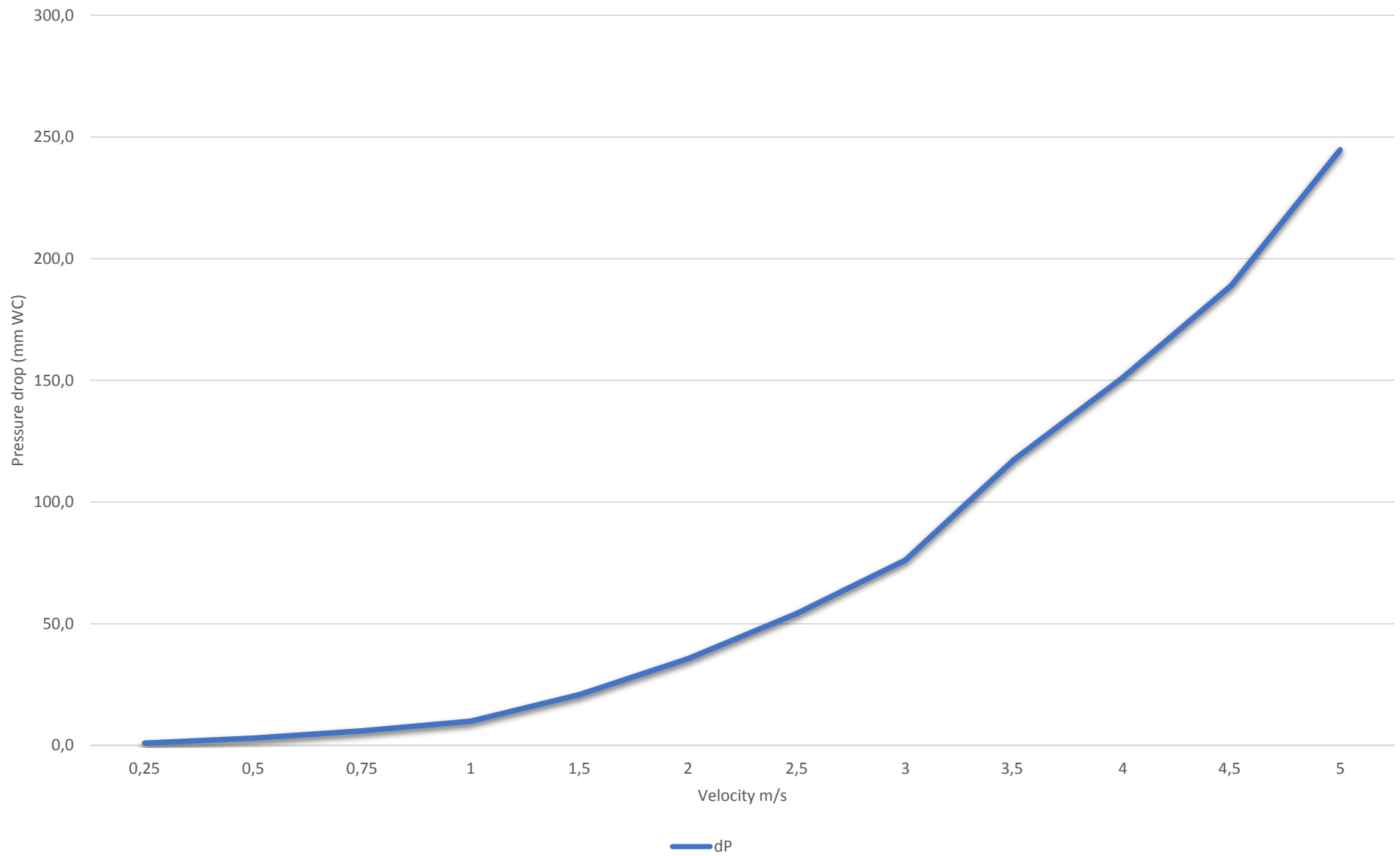
Pressure drop in function of velocity for BlueFil® MX99-2μ
