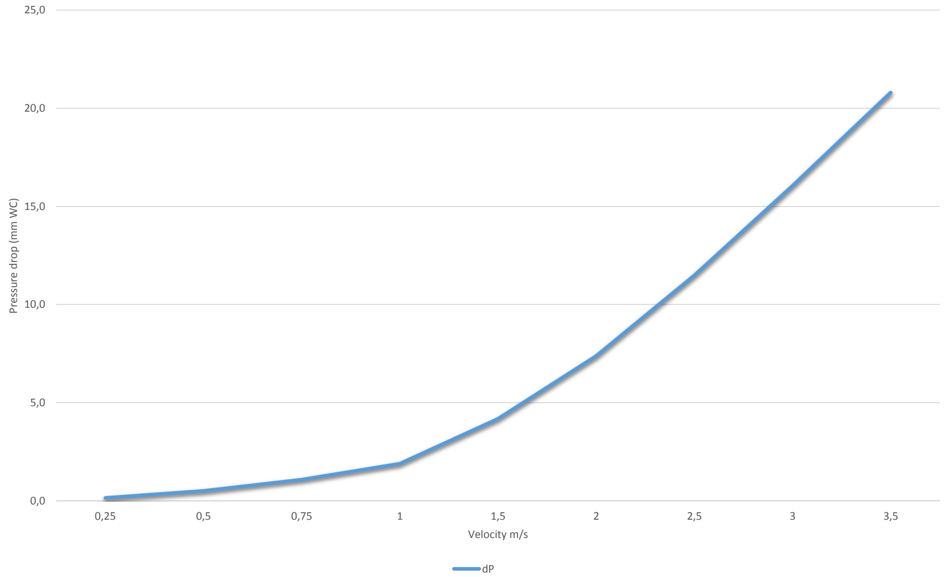
Pressure drop in function of velocity BlueFil® MX99-10
